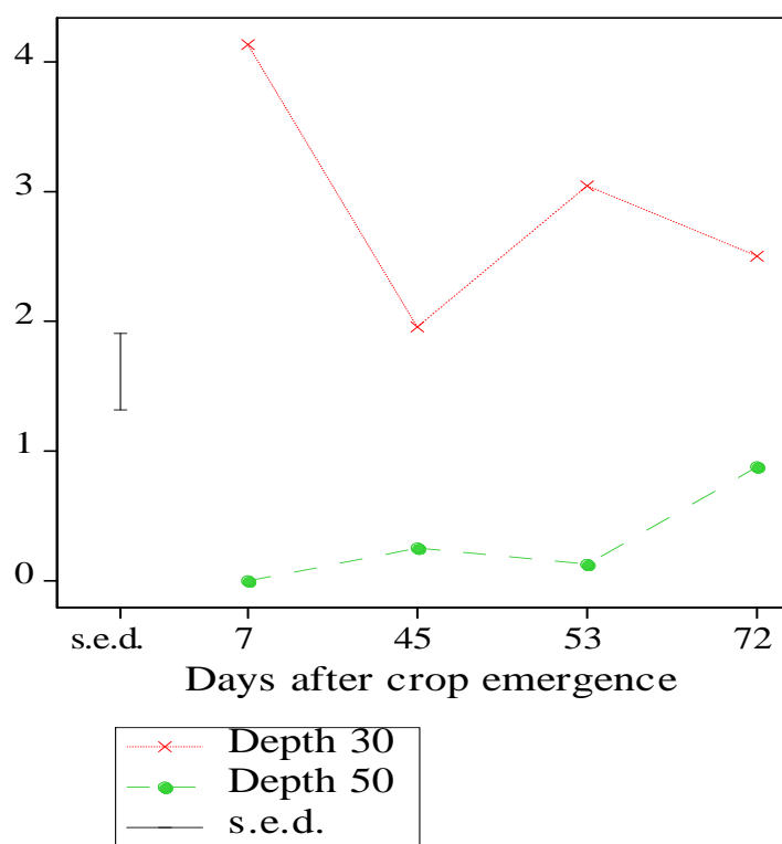
Figure 4.16 Interaction between profile depth and time with respect to phosphate concentrations ( \text{mg L}^{-1} ).
