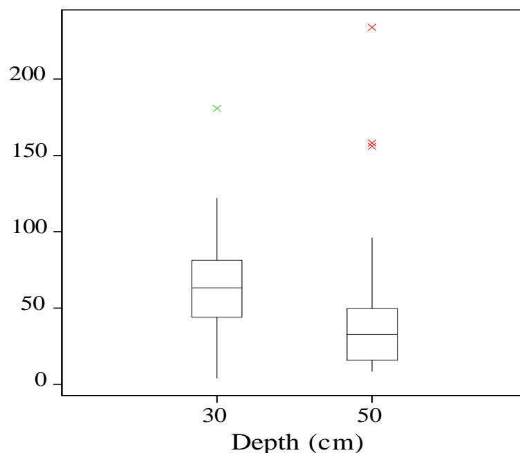
Figure 4.12 Nitrate concentrations ( \text{mg L}^{-1} ) at two soil depths 30 and 50 cm averaged over three irrigation treatments.
