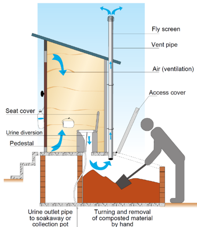
Figure 1: Schematic of a Urine Diversion Toilet (2)
